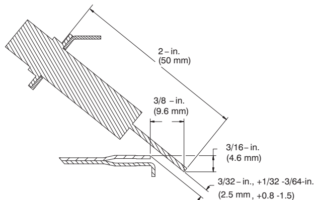
Figure 8 – Igniter Position – Side View
