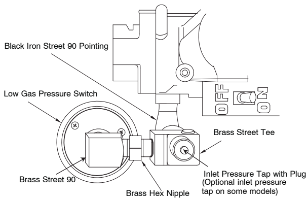
Figure 10 – Low Gas Pressure Switch Removal
