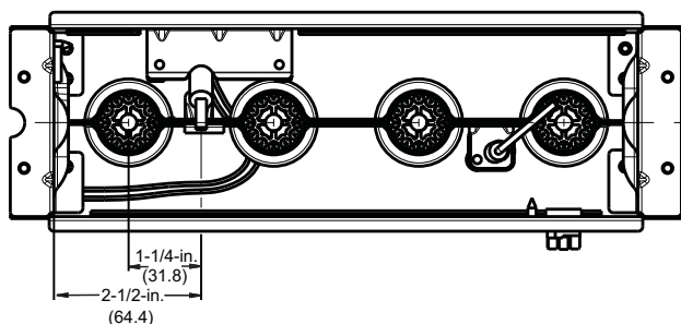
Figure 7 – Igniter Position – Back View
