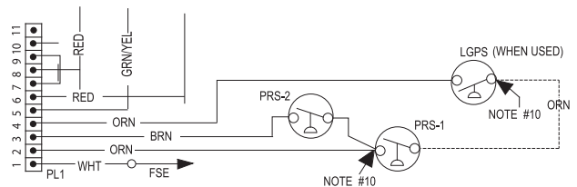
Figure 11 – Pressure Switch Wiring
