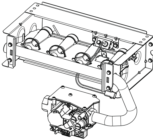
Fig. 1 - Burner Assembly / Manifold Assembly / Gas Valve
