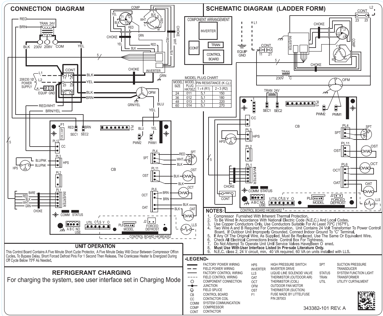
Fig. 1 – Wiring Diagram — 180CNV Model sizes 2 - 5 tons, 208/230-1
