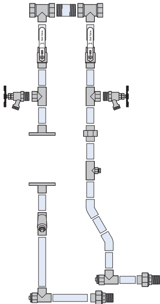
FIELD FABRICATED INSTALLATION
