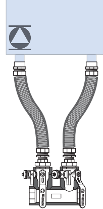
Wall Hung Boilers w/ Integral Pump
